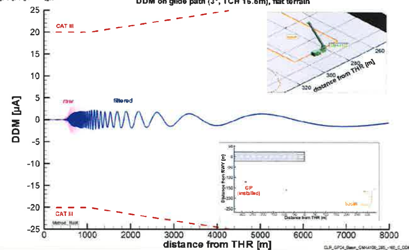
Airport Charleroi - GP24 Stormwater Basin position of crane GMK4100: 265m/-165m/0° DDM on glide path (3°, TCH 16.6m), flat terrain
